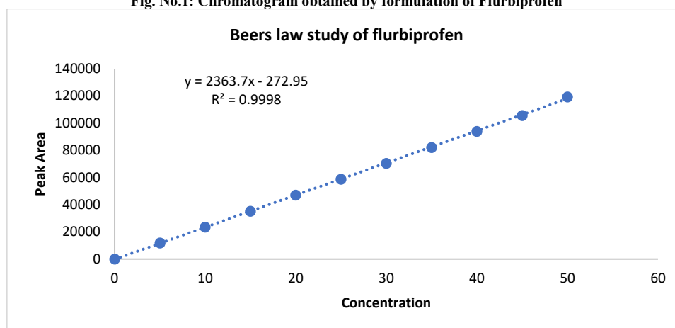
Fig.no.2: Linearity and range study for Flurbiprofen
