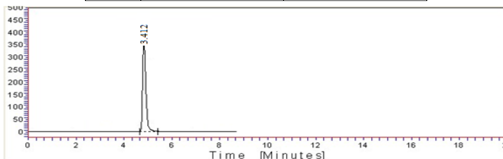
Fig. No.1: Chromatogram obtained by formulation of Flurbiprofen
