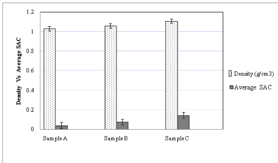
Figure 3.2 Influence of density on Sound absorption
