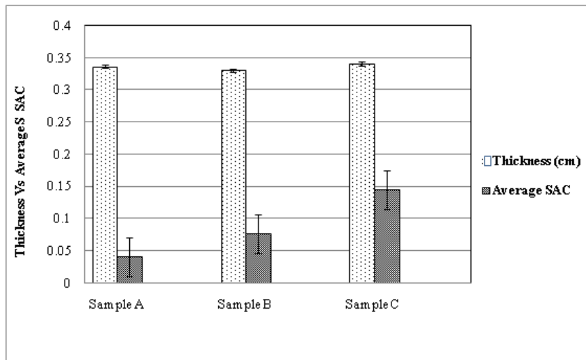
Figure 3 Thickness effect on Sound absorption
