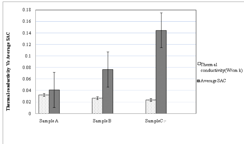
Figure 3.2.1 Influence of Sound Absorption on Thermal Conductivity
